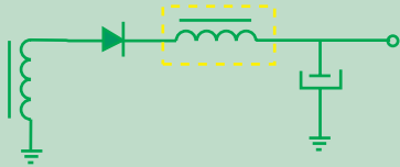
output choke
